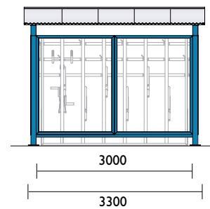
End Elevation / Section 3400
