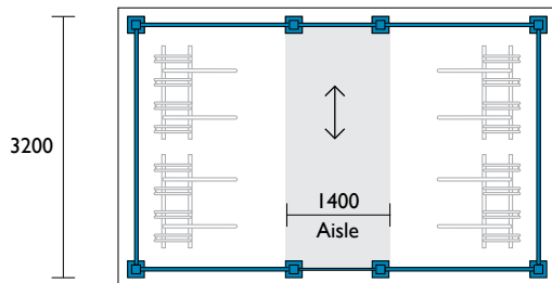
Plan View 5300
